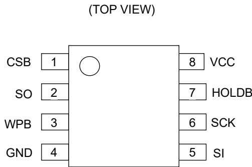
Figure 3. 端子配置図 (SOP8 *1 、SOP-J8、TSSOP-B8) *1 Last Time Buy.
