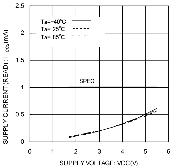
Figure 16. READ 動作時消費電流 I cc2 (READ, f SK =3MHz)
