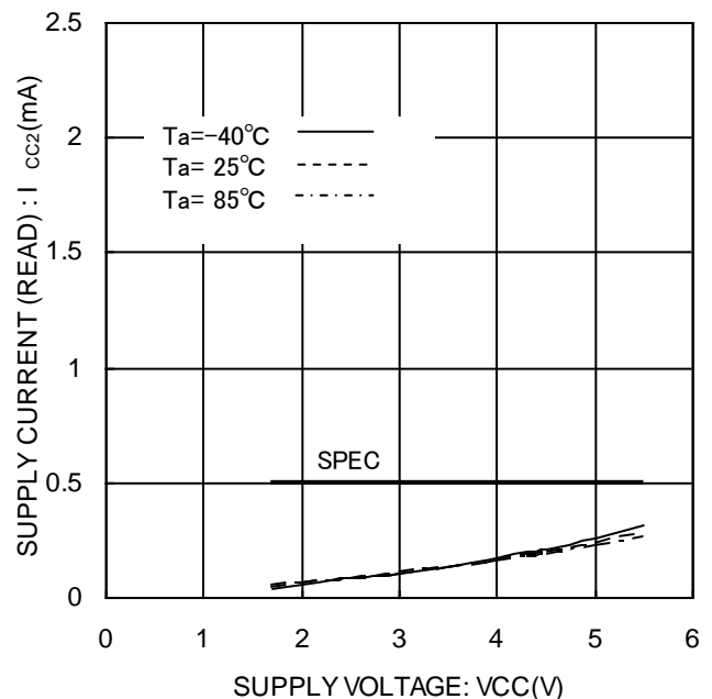
Figure 15. READ 動作時消費電流 I CC2 (READ, f SK =1MHz)
