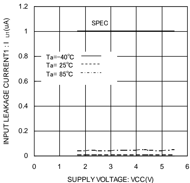
Figure 10. 入力リーク電流 1 I_{L1}(CS,SK,DI)
