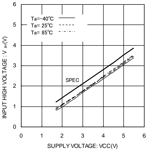
Figure 4. "H"入力電圧 V_{IH} (CS,SK,DI,ORG)
