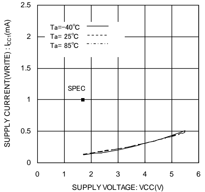
Figure 13. WRITE 動作時消費電流 I CC1 (WRITE, f SK =1MHz)
