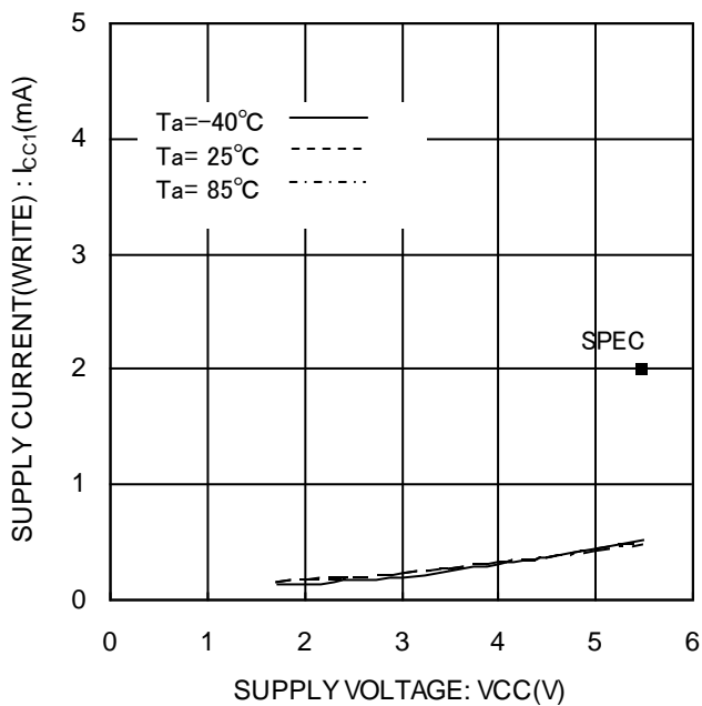
Figure 14. WRITE 動作時消費電流 I CC1 (WRITE, f SK =3MHz)
