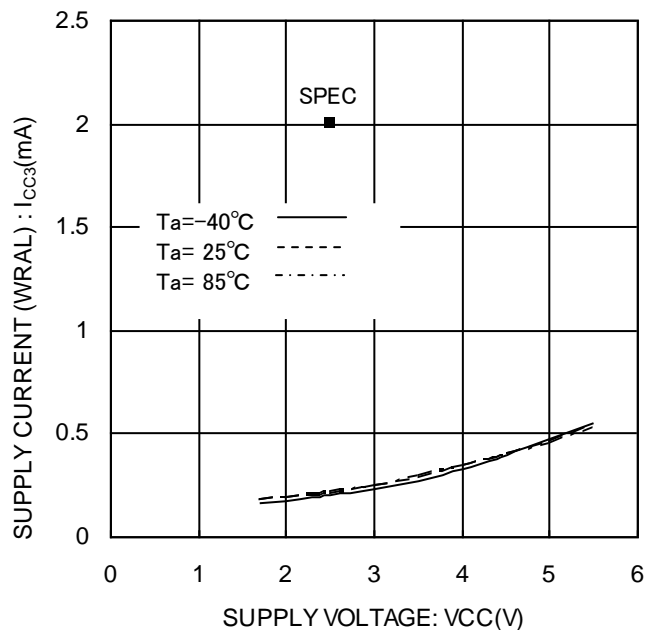
Figure 17. WRAL 動作時消費電流 I cc3 (WRAL, f SK =1MHz)
