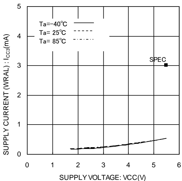
Figure 18. WRAL 動作時消費電流 I cc3 (WRAL, f SK =3MHz)
