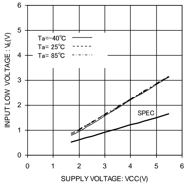
Figure 5. “L”入力電圧 V_{IL} (CS,SK,DI,ORG)
