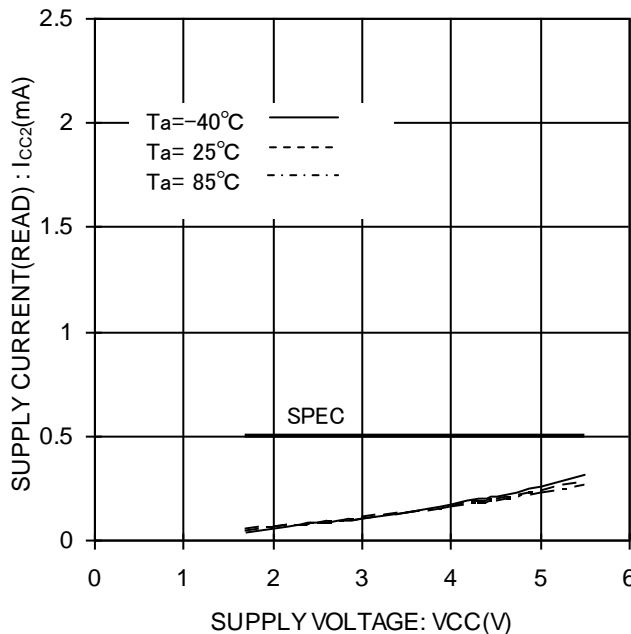
Figure 15. READ 動作時消費電流 I_{CC2}(READ, f_{SK}=1MHz)
