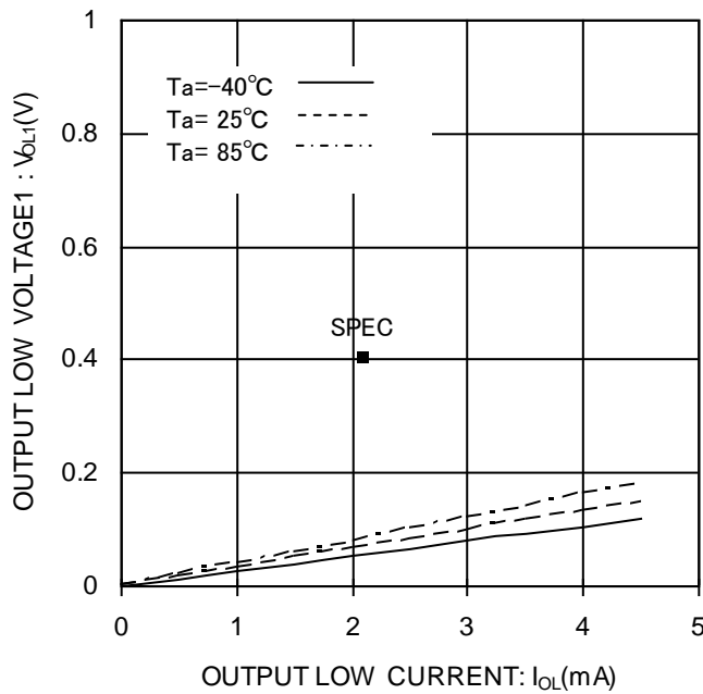
Figure 6. “L”出力電圧 1 V_{OL1} (VCC=2.7V)
