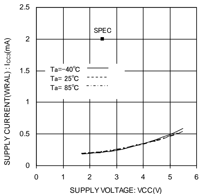
Figure 17. WRAL 動作時消費電流 Icc3(WRAL, fsk=1MHz)
