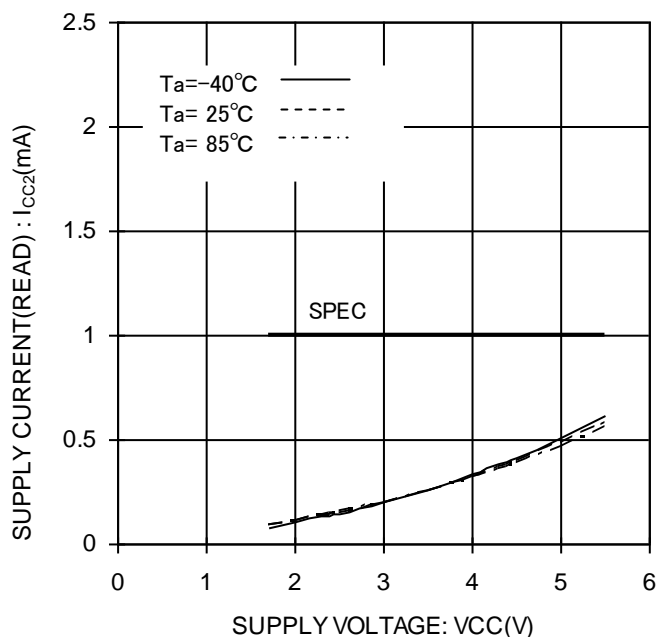
Figure 16. READ 動作時消費電流 Icc2(READ, fsk=3MHz)
