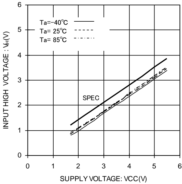
Figure 4. “H”入力電圧 V_{IH} (CS,SK,DI,ORG)
