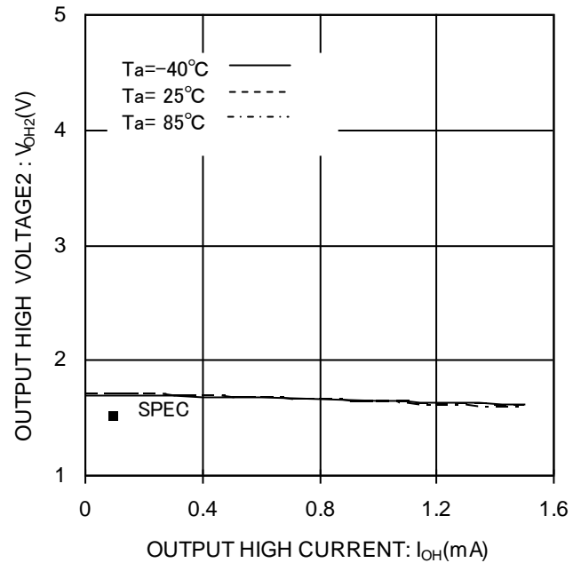
Figure 9. “H”出力電圧 2 V_{OH2}(VCC=1.7V)
