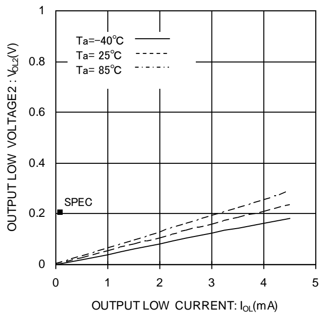
Figure 7. “L”出力電圧 2 V_{OL2} (VCC=1.7V)
