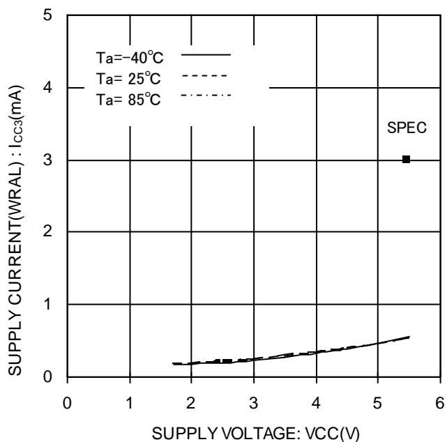
Figure 18. WRAL 動作時消費電流 Icc3(WRAL, fsk=3MHz)
