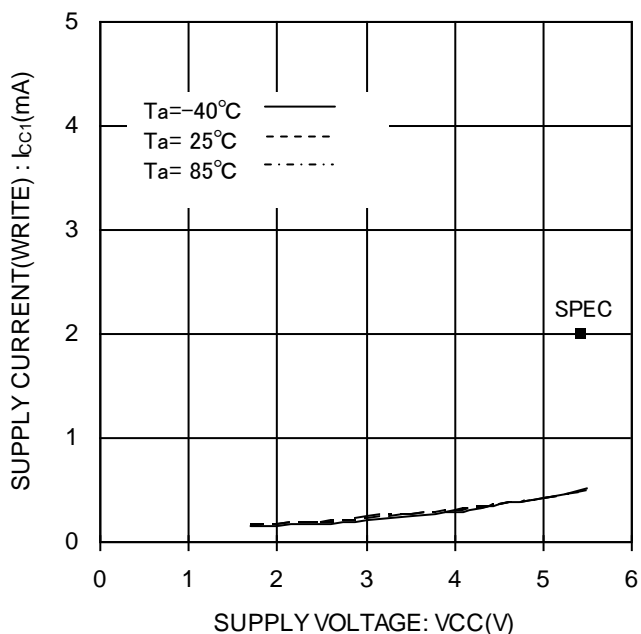
Figure 14. WRITE 動作時消費電流 I_{CC1}(WRITE, f_{SK}=3MHz)
