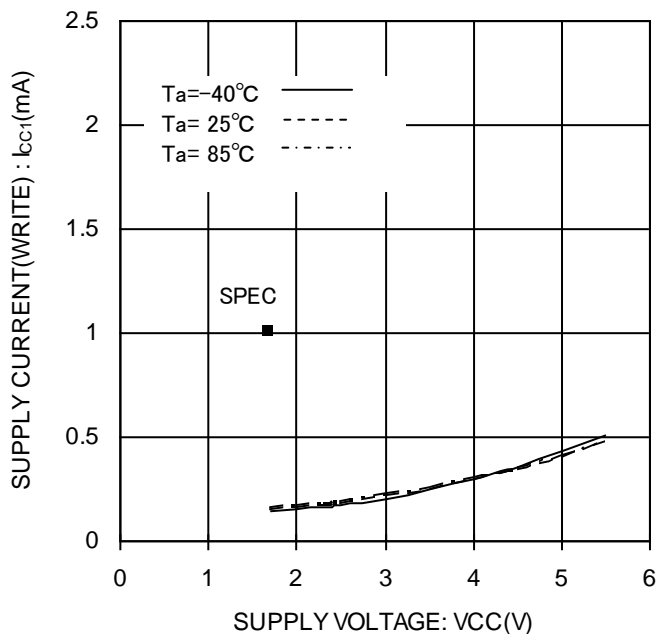
Figure 13. WRITE 動作時消費電流 I_{CC1}(WRITE, f_{SK}=1MHz)
