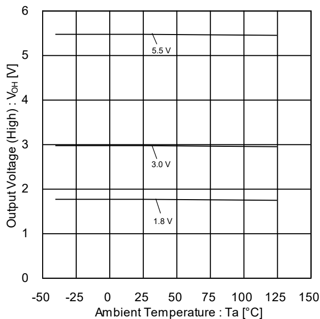
Figure 6. Output Voltage (High) vs Ambient Temperature ( R_L=10\text{ k}\Omega )
