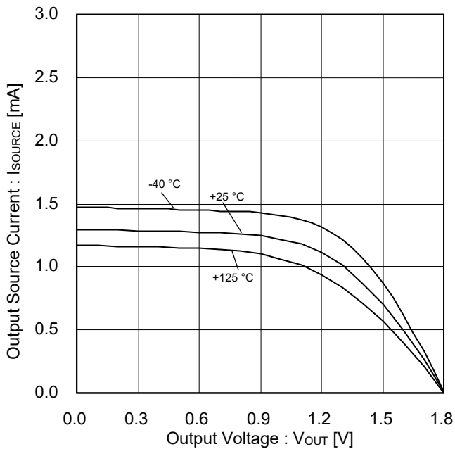
Figure 11. Output Source Current vs Output Voltage ( V_{DD}=1.8 V)
