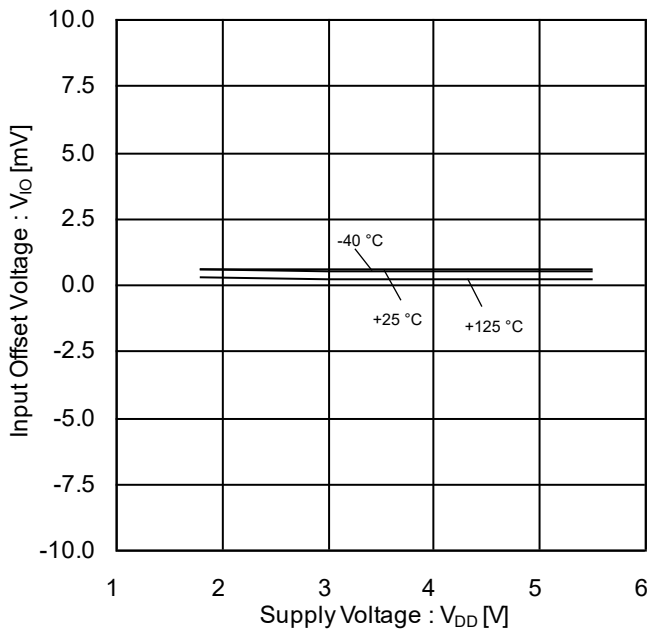
Figure 3. Input Offset Voltage vs Supply Voltage ( V_{ICM}=V_{DD} , E_K=-V_{DD}/2 )
