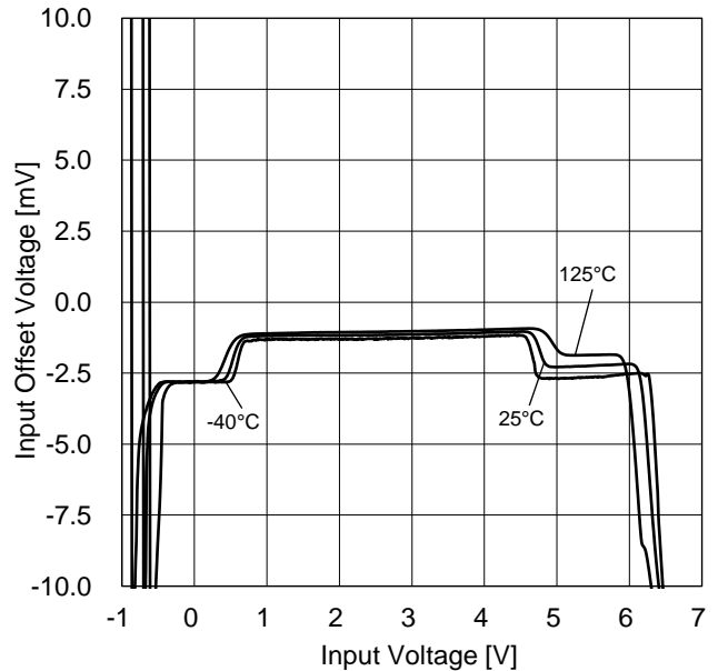
Figure 17. 同相入力電圧範囲 ( V_{DD}=5.5V )
