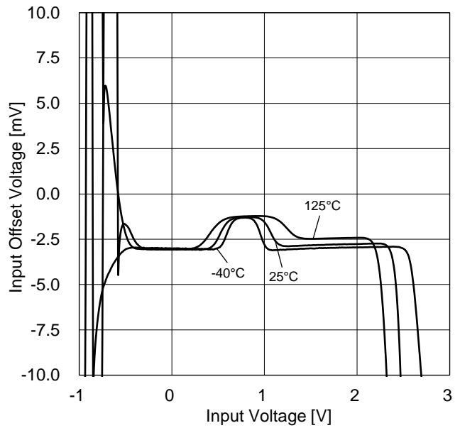
Figure 15. 同相入力電圧範囲 ( V_{DD}=1.8V )
