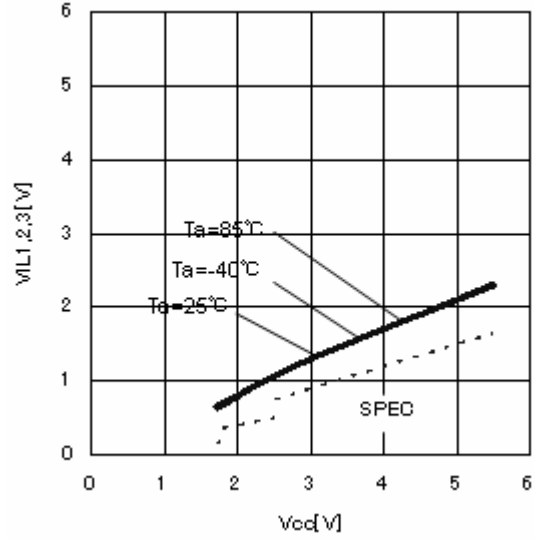
Figure 3. L input voltage V_{LI1, 2, 3} (A2, SCL, SDA, WP)
