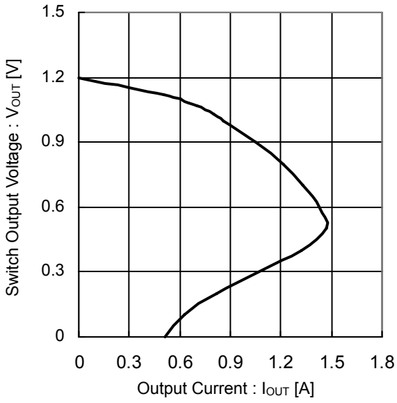
Figure 22. Switch Output Voltage vs Output Current (V IN =1.2V)
