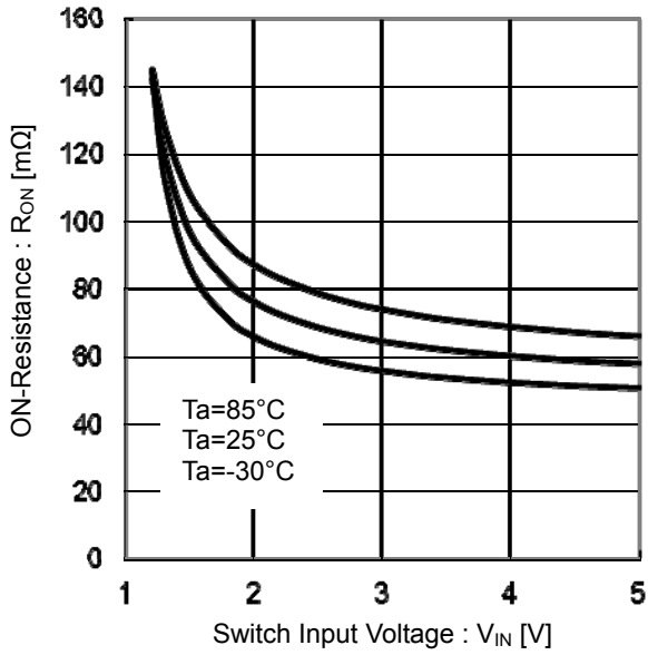
Figure 6. ON-Resistance vs Switch Input Voltage
