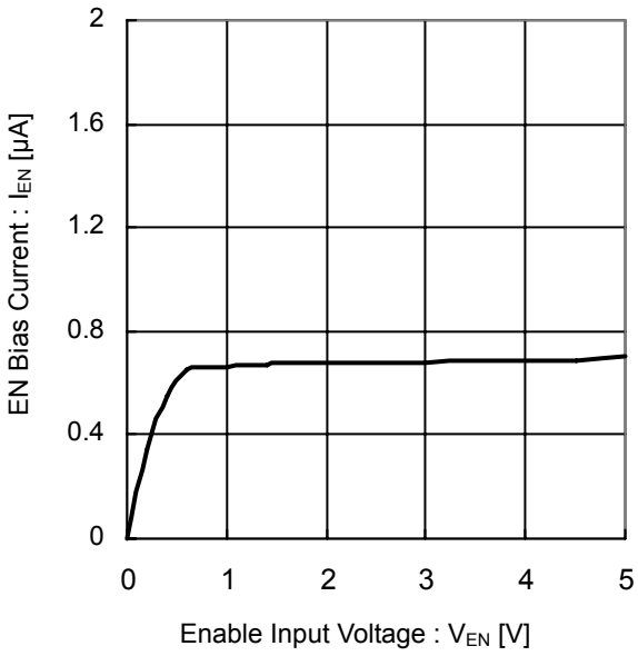
Figure 18. EN Bias Current vs Enable Input Voltage
