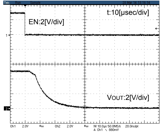
Figure.59 Turn off response 12 (BUS1DJC3GWZ V_{IN}=5V )
