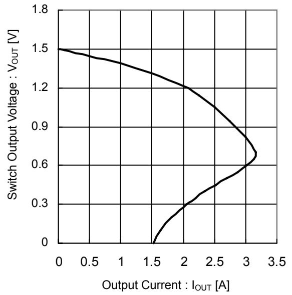
Figure 23. Switch Output Voltage vs Output Current (V IN =1.5V)
