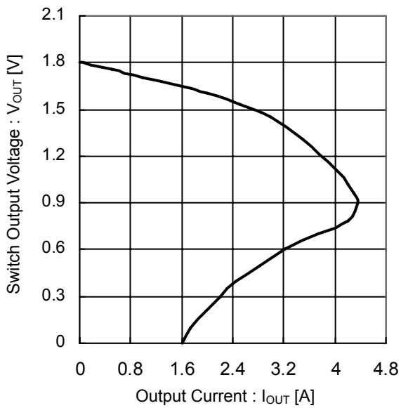
Figure 24. Switch Output Voltage vs Output Current (V IN =1.8V)
