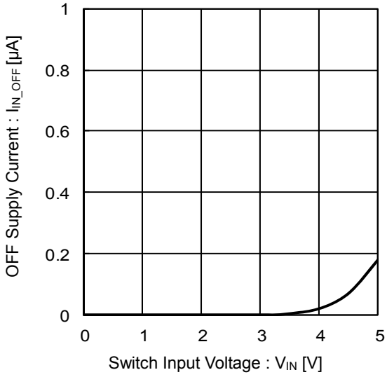
Figure 10. OFF Supply Current vs Switch Input Voltage ( V_{EN}=0V )
