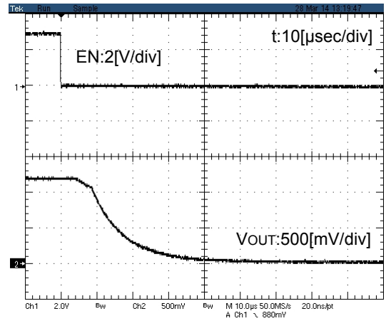
Figure.49 Turn off response 7 (BUS1DJC3GWZ VIN=1.2V)
