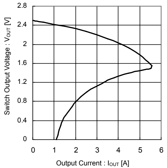
Figure 25. Switch Output Voltage vs Output Current (V IN =2.5V)
