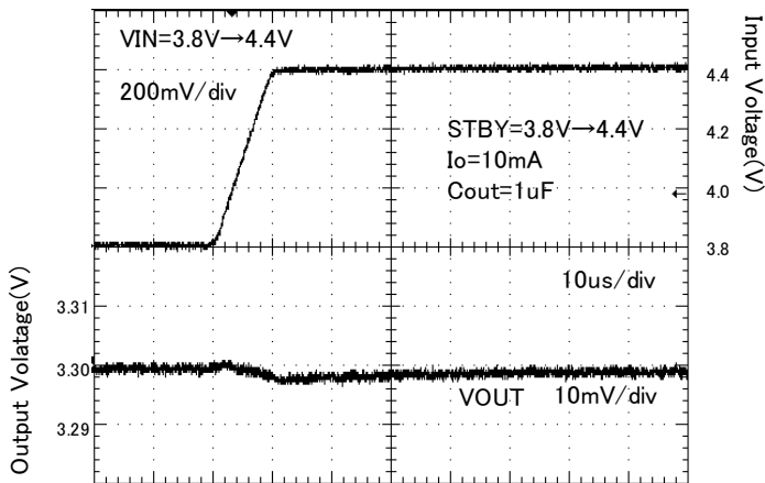
Figure 25. Line response ( V_{in} = 3.8\text{V} \rightarrow 4.4\text{V} )
