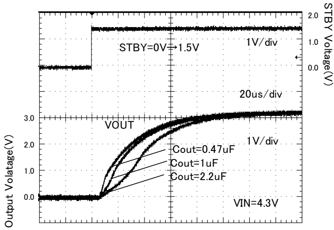
Figure 19. Startup time ( R_{out} = \text{none} )
