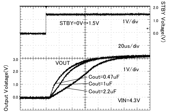
Figure 20. Startup time ( R_{out} = 16.5\ \text{ohm} )
