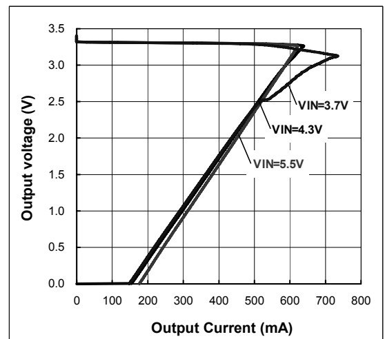
Figure 8. OCP Threshold
