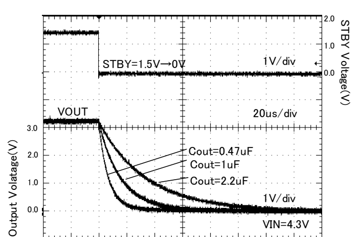
Figure 22. Discharge time ( R_{out} = 16.5\ \text{ohm} )
