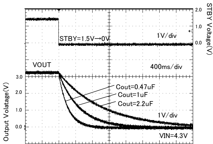
Figure 21. Discharge time ( R_{out} = \text{none} )
