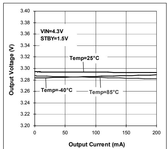
Figure 6. Load Regulation
