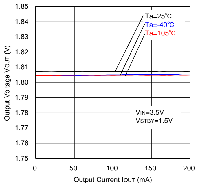
Figure 28. Load Regulation
