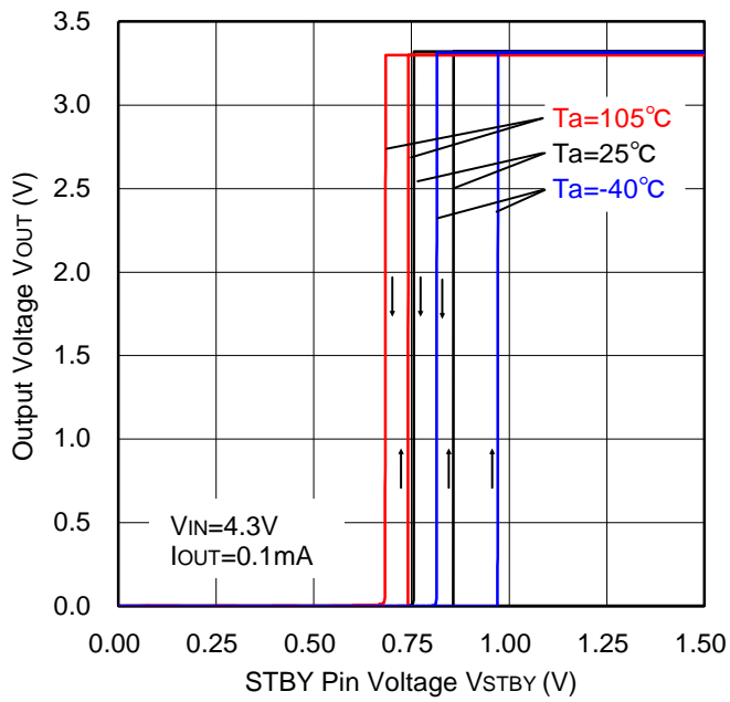
Figure 78. STBY Threshold
