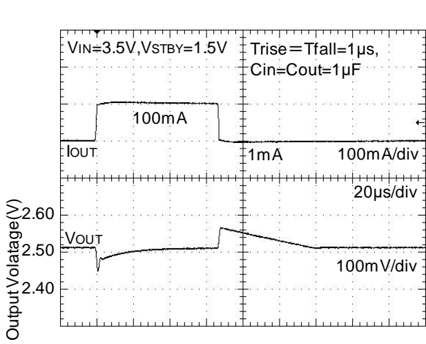
Figure 62. Load Response (1mA to 100mA)
