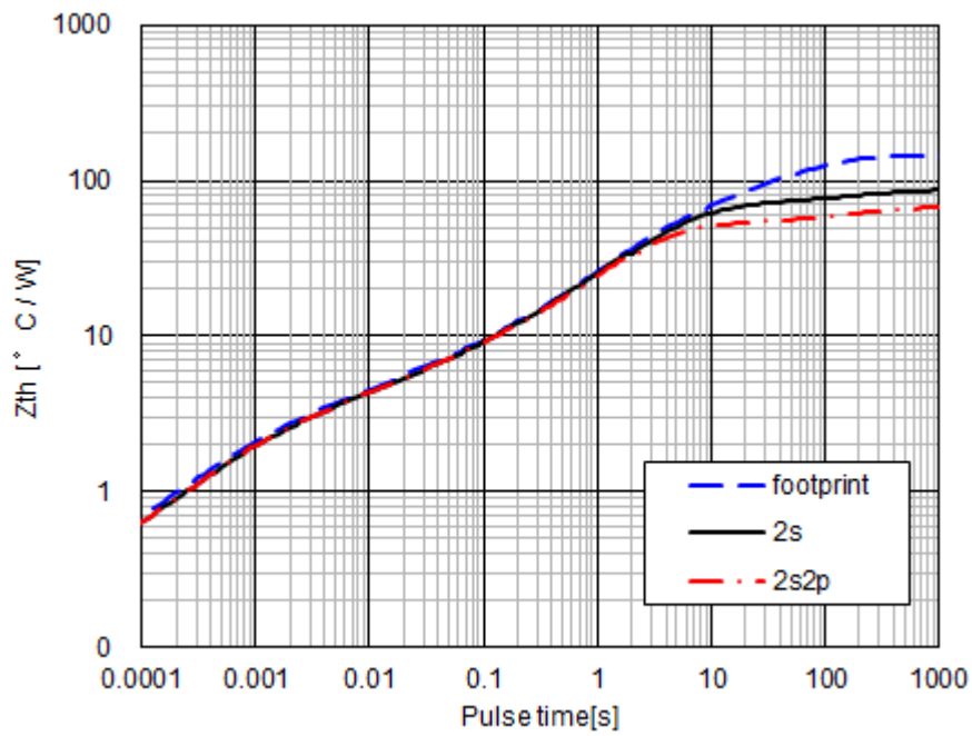
Figure 5. 過渡熱抵抗
