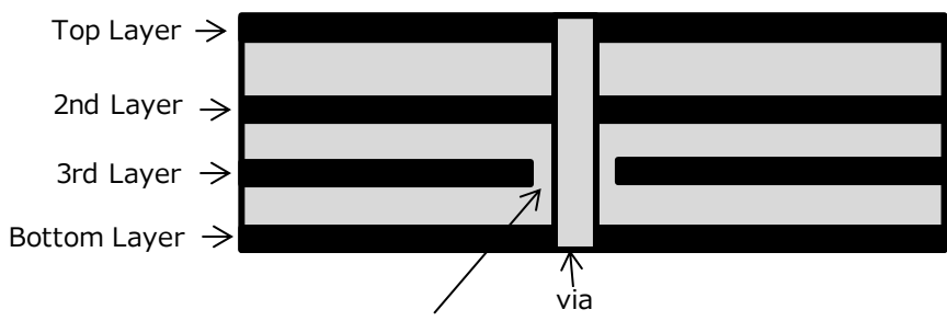
Cross Section
