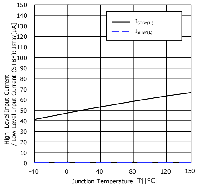
Figure 6. High Level Input Current / Low Level Input Current (STBY) vs Junction Temperature
