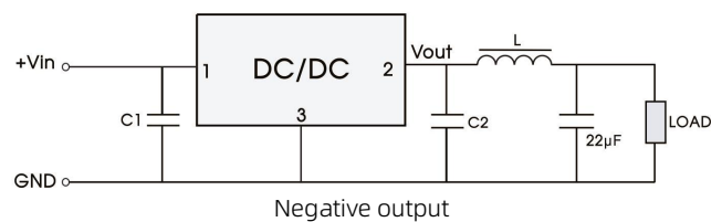
Fig. 4 Using the "LC" output filter application
