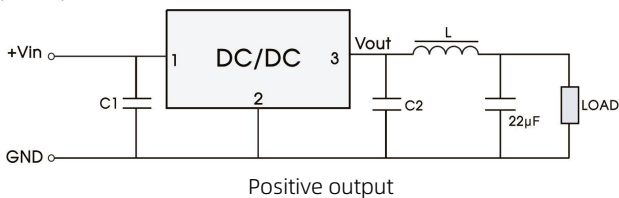
Fig. 4 Using the "LC" output filter application
