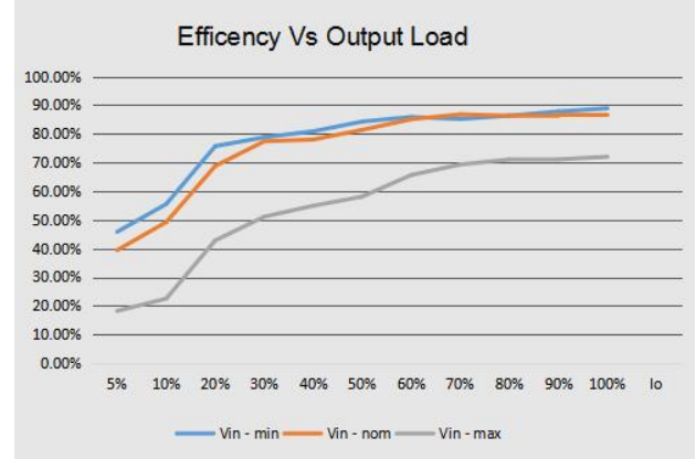
DRULD10-F1D54(F/H) Efficiency curve of output load (normal temperature)
