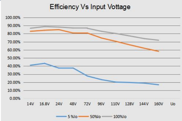
DRULD10-F1D54(F/H) Efficiency curve of input voltage (normal temperature)
