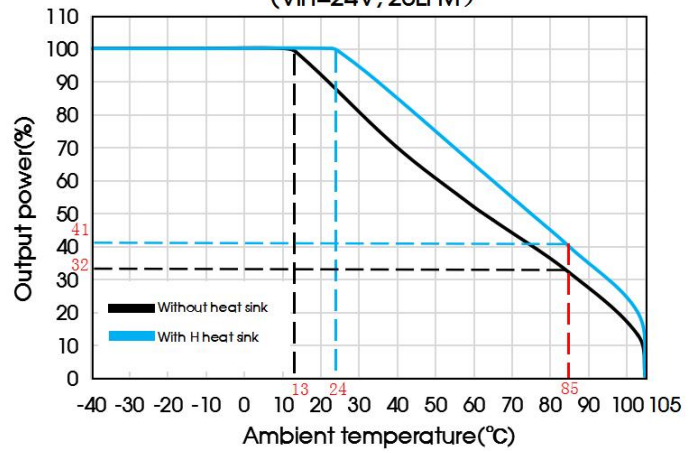
DRUQB100-F1D24 Temperature Derating Curves (Vin=24V, 20LFM)
