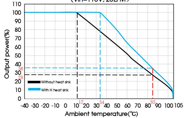
DRUQB100-F1D24 Temperature Derating Curves (Vin=110V, 20LFM)
