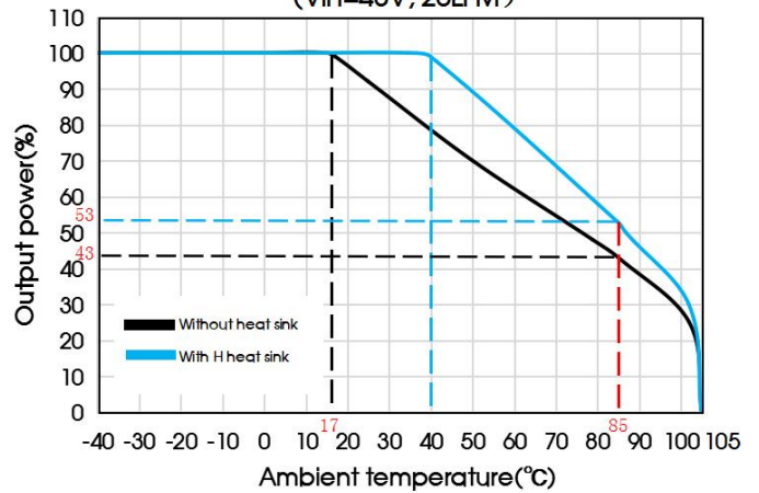
DRUQB100-F1D12 Temperature Derating Curves (Vin=48V, 20LFM)
