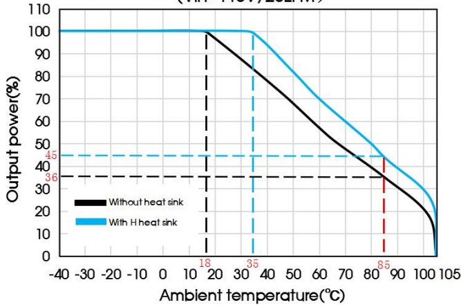
DRUQB100-F1D12 Temperature Derating Curves (Vin=110V, 20LFM)
