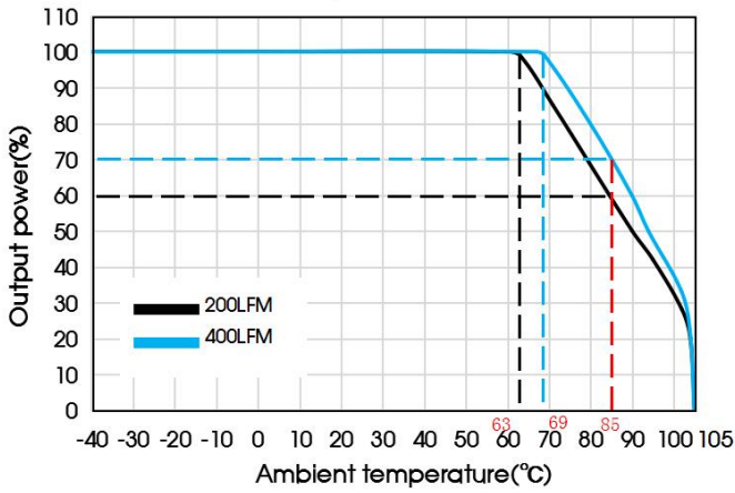
DRUQB100-F1D54H Temperature Derating Curves ( V_{in}=110V )
