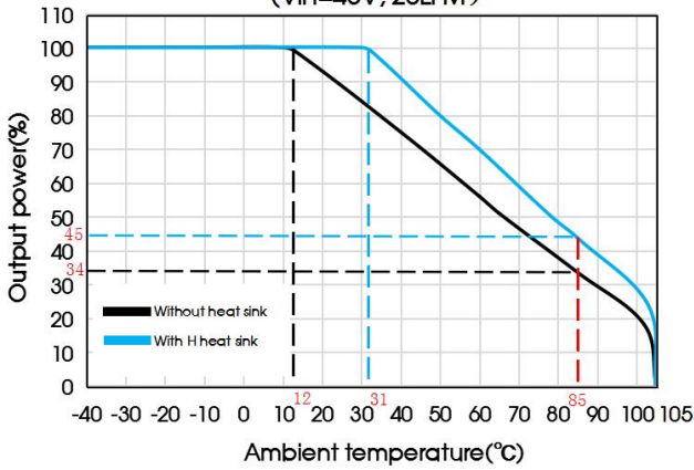
DRUQB100-F1D24 Temperature Derating Curves (Vin=48V, 20LFM)
