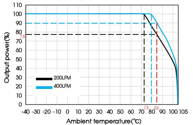
DRUQB100-F1D54H Temperature Derating Curves (Vin=48V)
