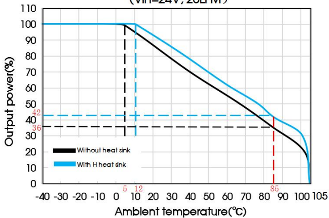
DRUQB100-F1D12 Temperature Derating Curves (Vin=24V, 20LFM)
