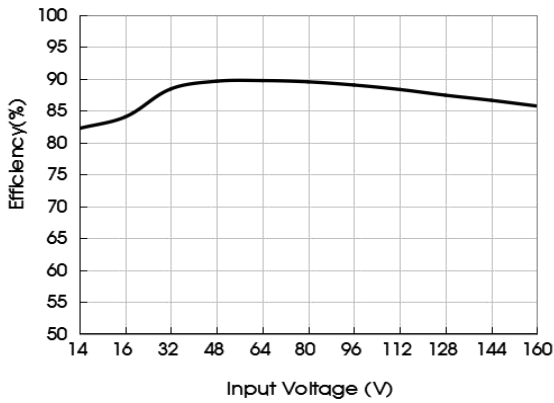
Efficiency Vs Input Volyage (Full Load)
