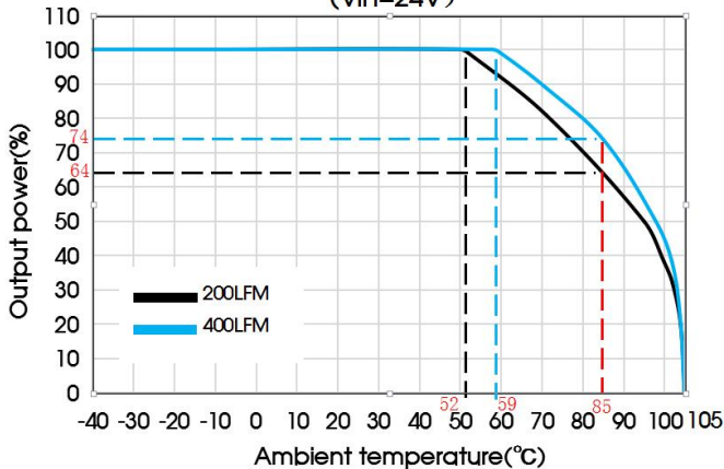
DRUQB100-F1D54H Temperature Derating Curves (Vin=24V)
