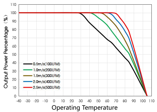
DRWHB250-F1D54H Temperature Derating Curve
