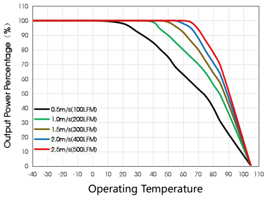
DRWHB250-F1D15H Temperature Derating Curve
