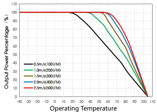
DRWHB250-F1D54H Temperature Derating Curve
