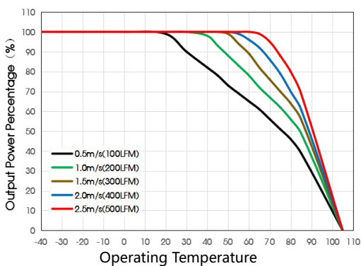
DRWHB250-F1D48H Temperature Derating Curve
