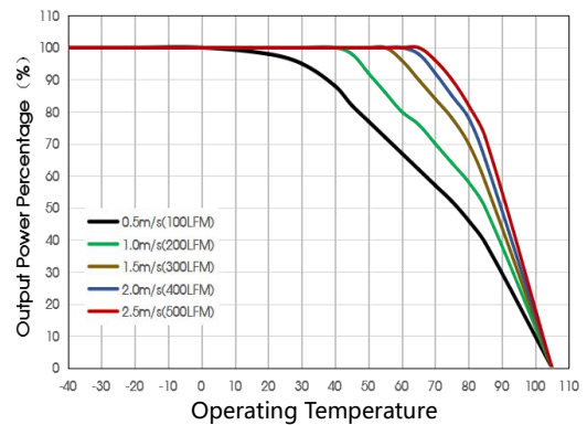
DRWHB250-F1D24H Temperature Derating Curve
