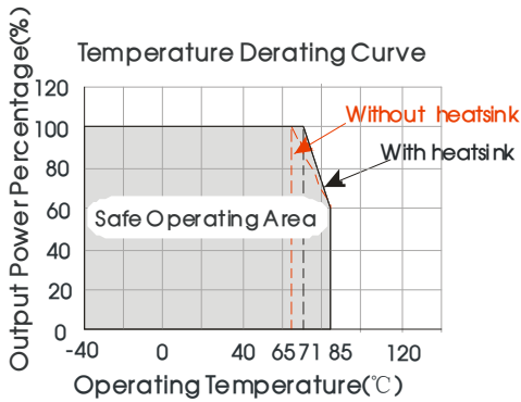
Operating Temperature, Except DRWLD20-B1D03/05(H)(E2S/D4S)
