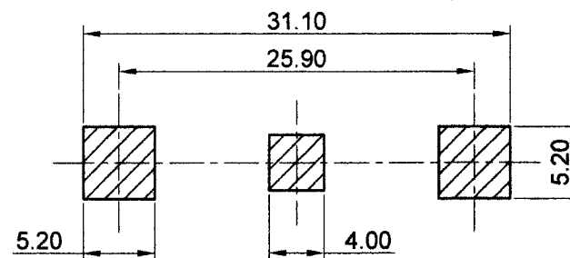
PCB MOUNTING LAYOUT
