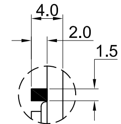
DETAIL "B" S=2:1 Polarity protection device
