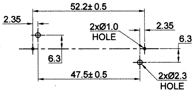
PCB/MOUNTING LAYOUT
