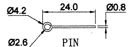
DETAIL "B" S=2:1 Polarity protection device
