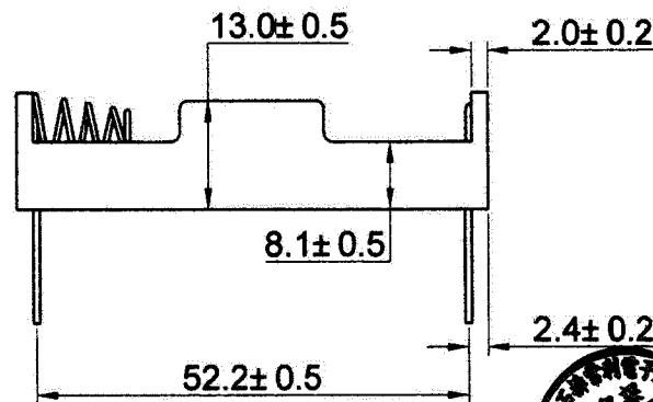
DETAIL "B" S=2:1 Polarity protection device
