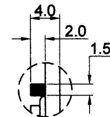
DETAIL "B" S=2:1 Polarity protection device
