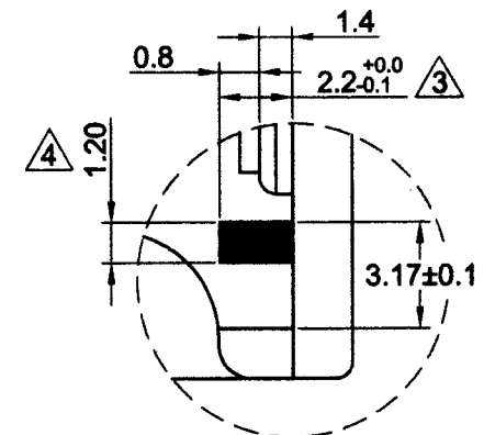
DETAIL "A" S=4 POLARITY PROTECTION DEVICE
