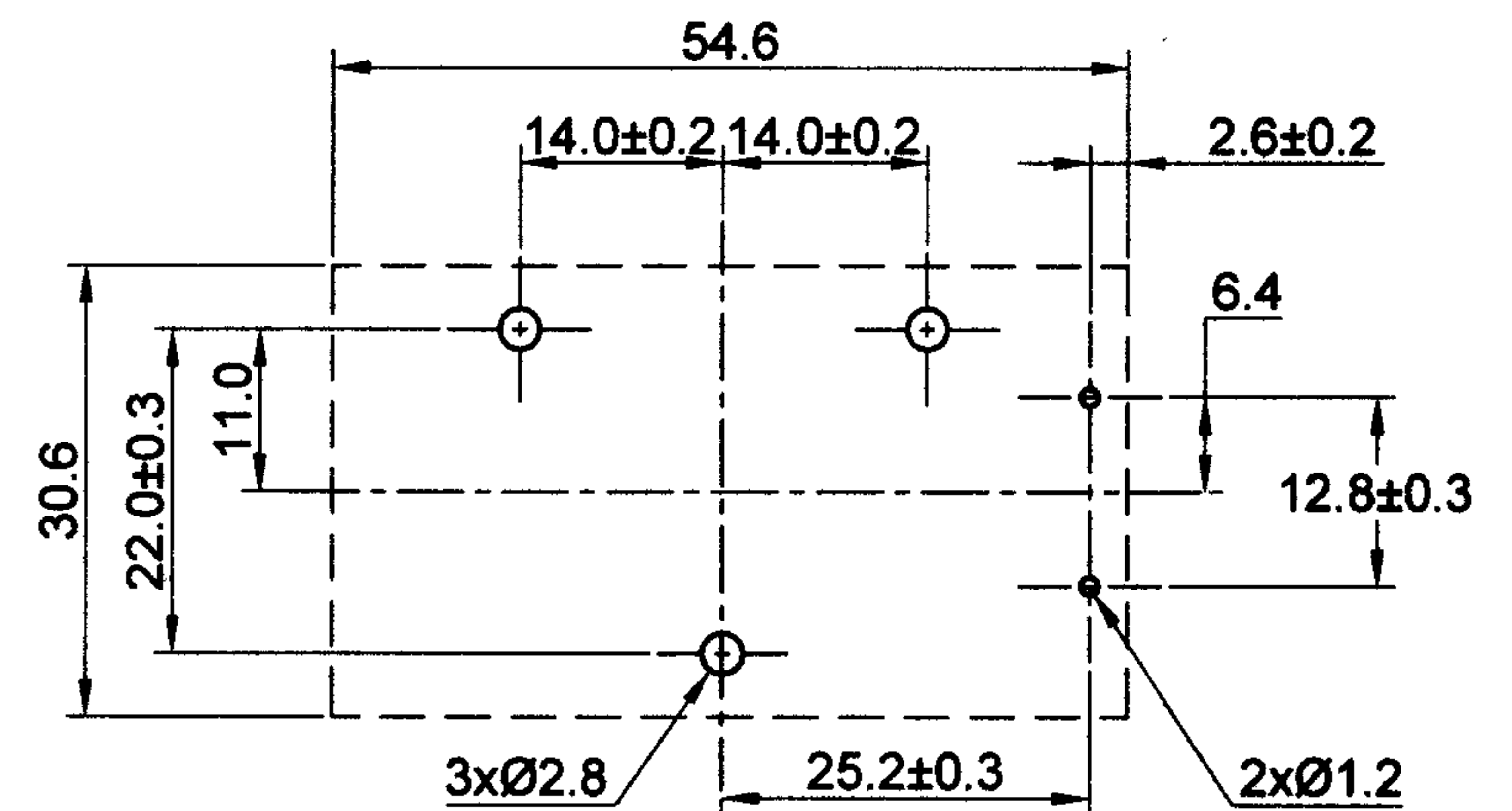
PCB/MOUNTING LAYOUT
