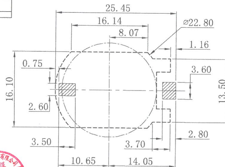
PCB MOUNTING LAYOUT
