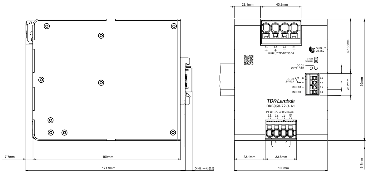
図.23: DRB960-72-3-A1の寸法図
