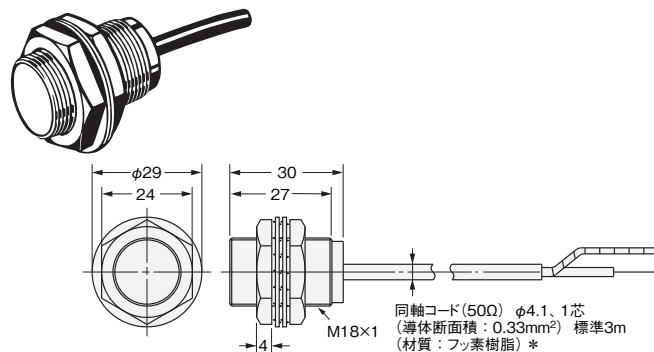
形E2C-X5AH *
