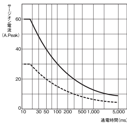
形G3NE-205T (L)
