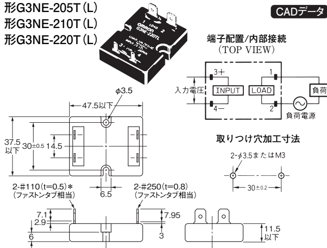
形G3NE-205T (L)
