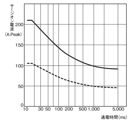
形G3NE-220T (L)
