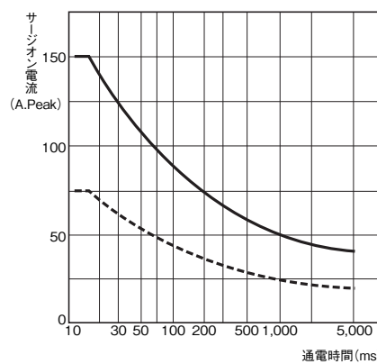
形G3NE-210T (L)
