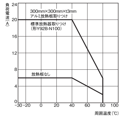
形G3NE-220T (L)
