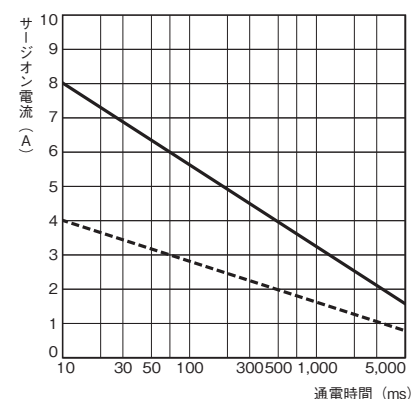
形G3R-ODX02SN
