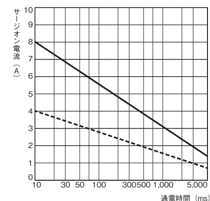
形G3R-OD201SN
