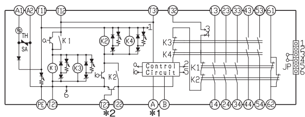
形G9SA-321-T□ (AC/DC24V)
