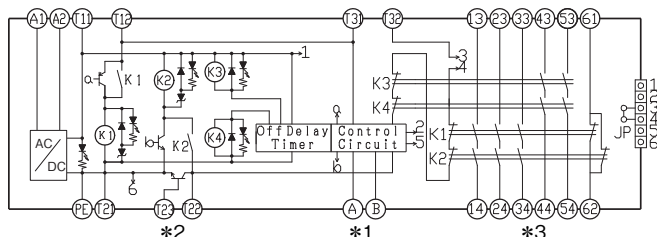
形G9SA-TH301 (AC100~240V)
