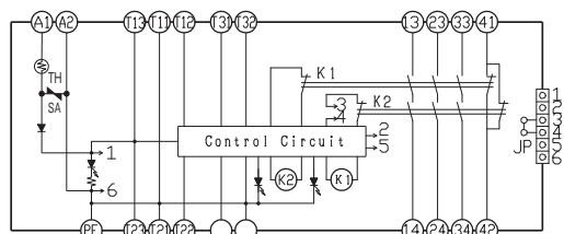
形G9SA-TH301 (AC/DC24V)
