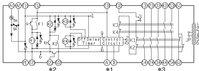
形G9SA-TH301 (AC/DC24V)
