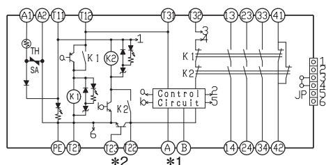
形G9SA-501 (AC/DC24V)
