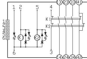
形G9SA-EX301
