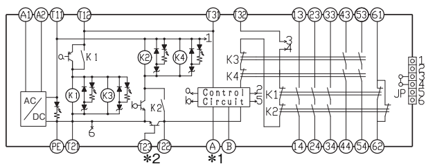
形G9SA-321-T□ (AC100~240V)
