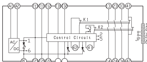
形G9SA-TH301 (AC100~240V)
