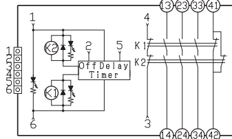
形G9SA-EX031-T□
