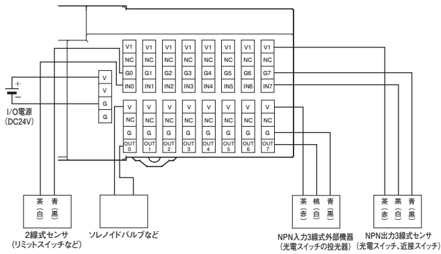
形GX-MD3218(NPN対応)
