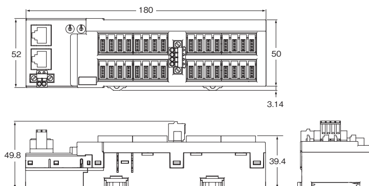
形GX-MD3218/MD3228
