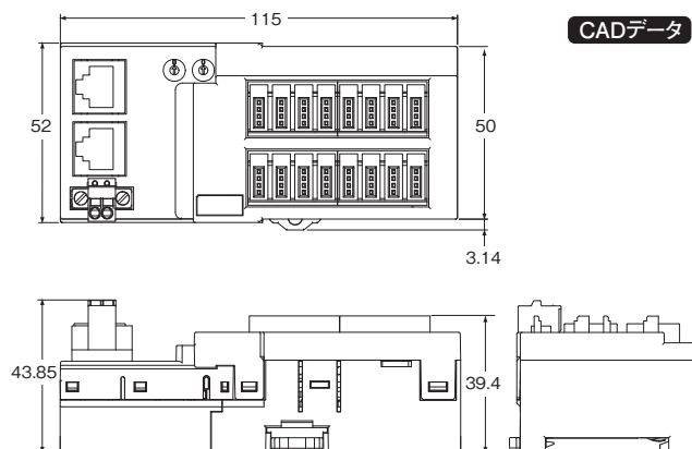
形GX-ID3218/ID3228
