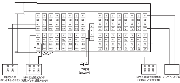
形GX-MD3218(NPN対応)
