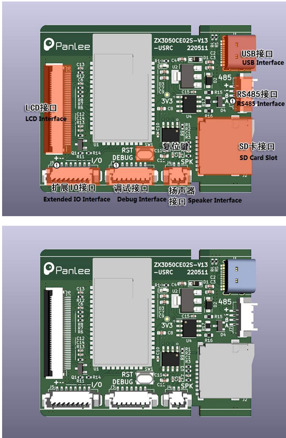
Fig.1 Hardware Interface
