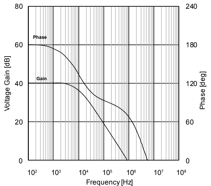
Figure 53. 電圧利得・位相–周波数特性 (V CC =30V, R L =2kΩ, C L =100pF)
