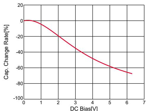
GRM188B30J475KE18#, C-DC bias, capchange, 20.0degC, AC0.5Vrms
