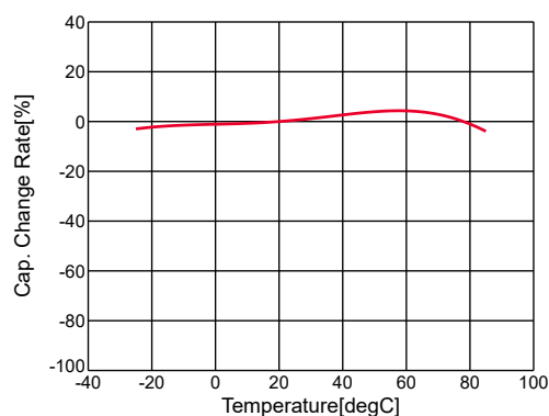
GRM188B30J475KE18#, C-Temp., capchange, DC0.0V, AC0.3Vrms
