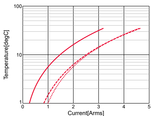
GRM188B30J475KE18#, Temp.rise
