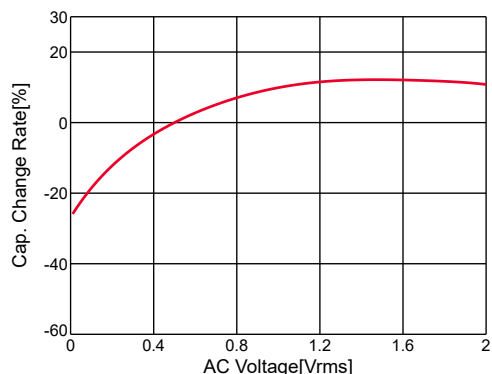
GRM188B30J475KE18#, C-AC Voltage, capchange, DC0V, 20.0degC
