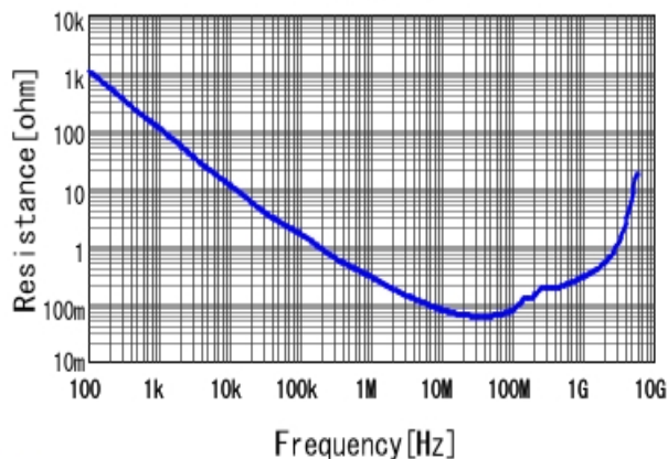
■ GRM188B11H103KA01 R DCOV, 20degC
