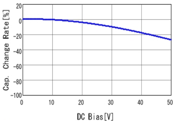
■ GRM188B11H103KA01 C-DC bias capchange, 20.0degC, AC1.
