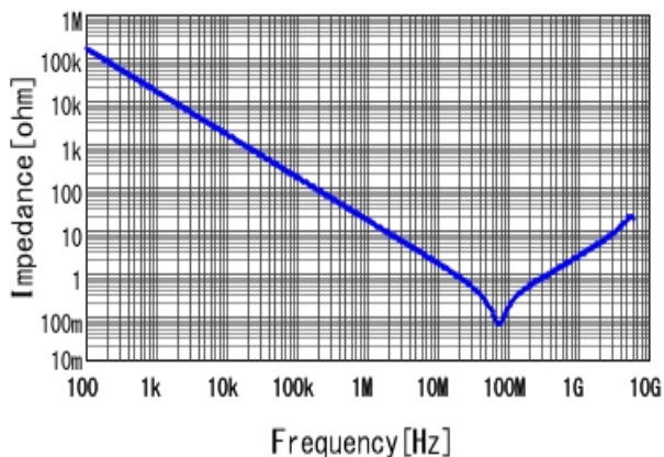
■ GRM188B11H103KA01 |Z| DCOV, 20degC
