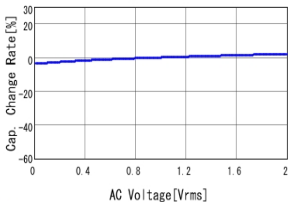
■ GRM188B11H103KA01 C-AC Voltage capchange, DCOV, 20.0d
