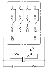
形MY4(Z) IN-CR(S) (AC仕様のみ)
