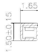
Section:C-C
