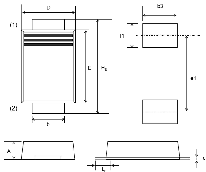
SOD-128, (PMDTM)
