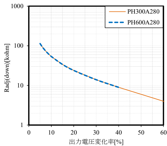
図7-6 外付け抵抗(Radj(down)) 対 \Delta(\%)
