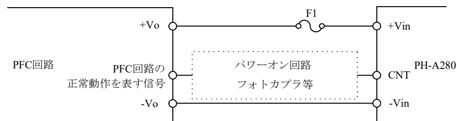
図7-20 CNT接続例(3)
