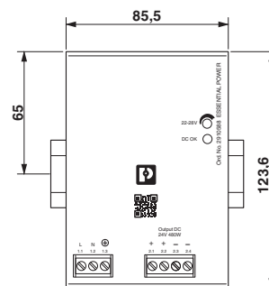
Dimensional drawing
