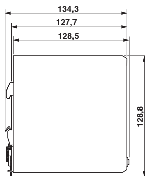
Dimensional drawing
