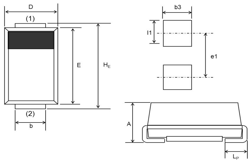
DO-214AC(SMA), (PMDS)
