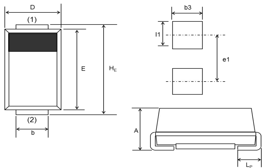
DO-214AC(SMA), (PMDS)
