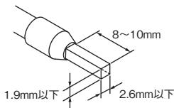
形PYF-□□-PU/形P2RF-□□-PU
