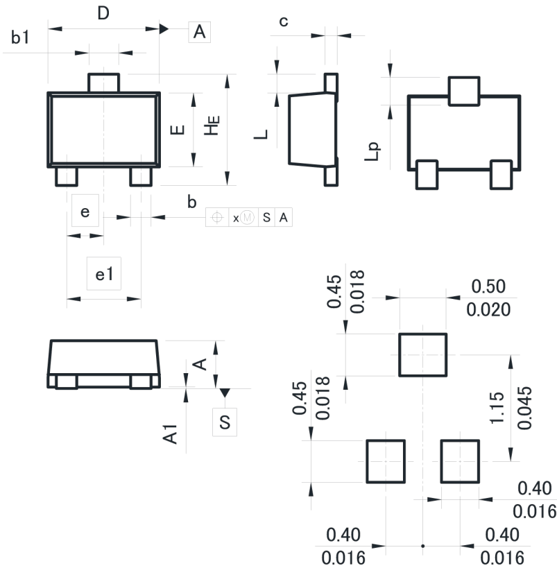
Soldering footprint Unit: ( \frac{\text{mm}}{\text{inches}} )
