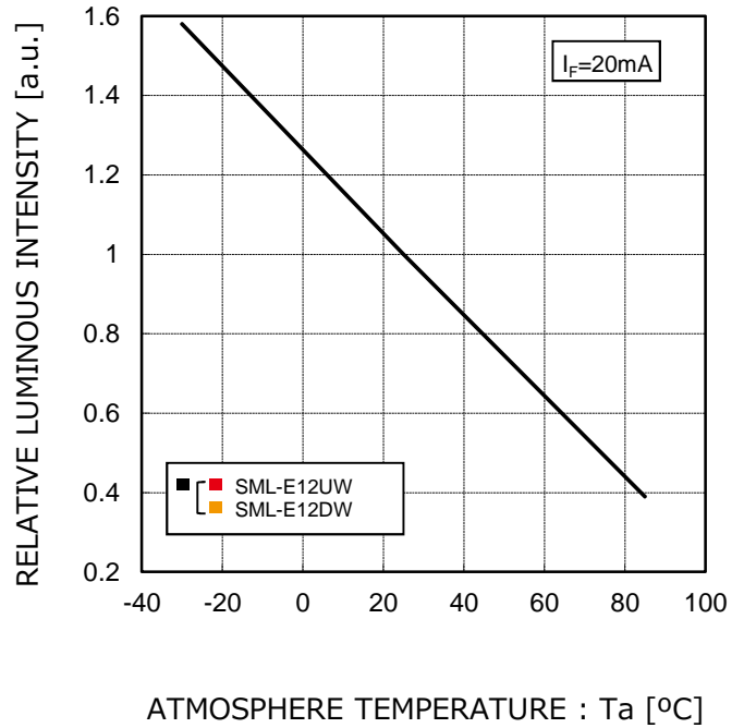
Fig.2 Luminous Intensity - Atmosphere Temperature
