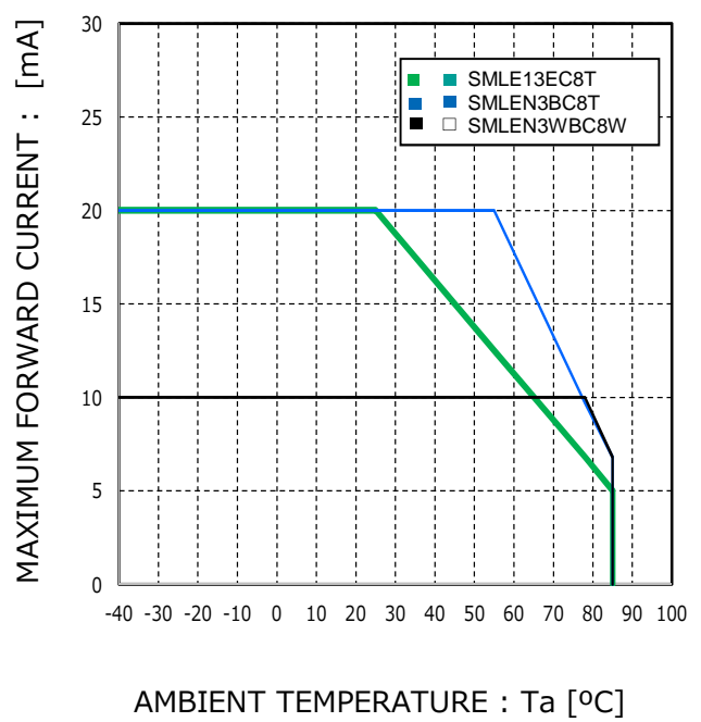
Fig.4 Derating
