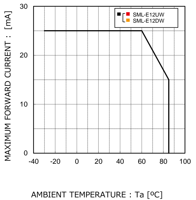
Fig.4 Derating
