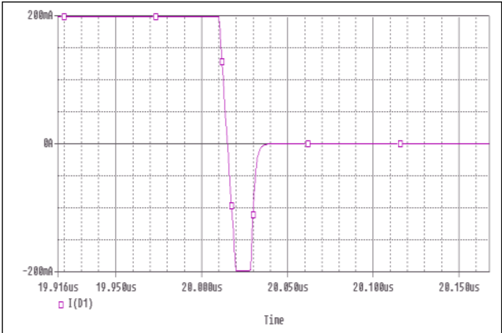
Circuit Simulation Result
