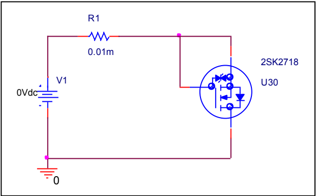
Evaluation Circuit
