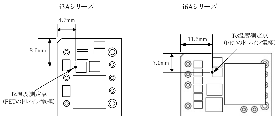
図6-6 Tc温度測定点 (Top View)
