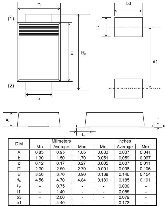
SOD-128, (PMDTM)
