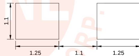
Soldering Pad
