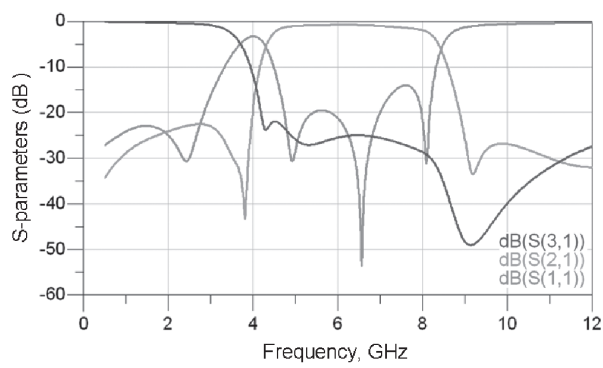
RFDIP160806ALM6T25
