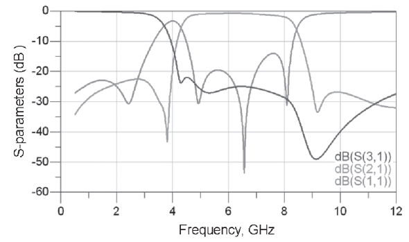
RFDIP1608060LVT
