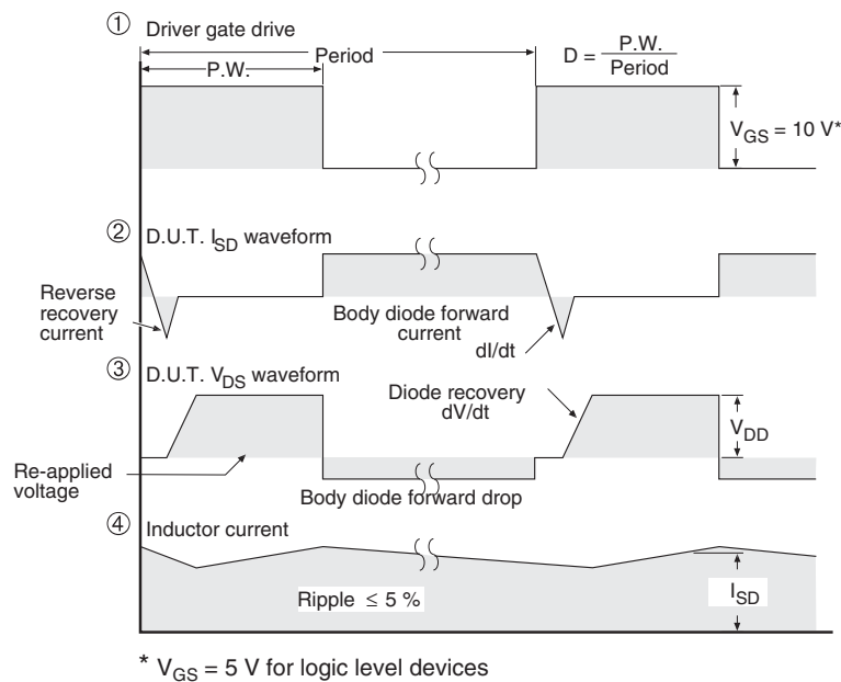
Fig. 11 - For N-Channel
