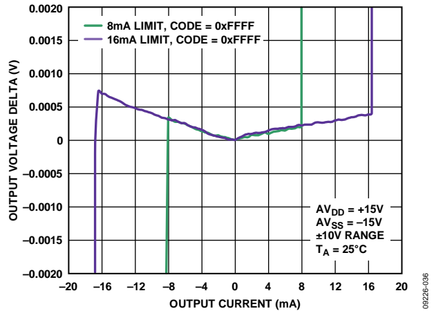
Figure 24. Source and Sink Capability of Output Amplifier
