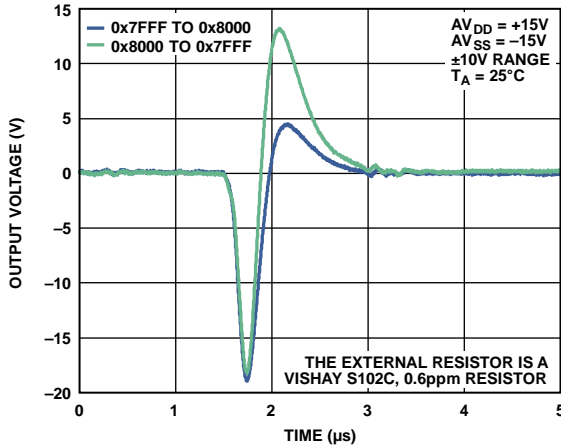
Figure 27. Digital-to-Analog Glitch
