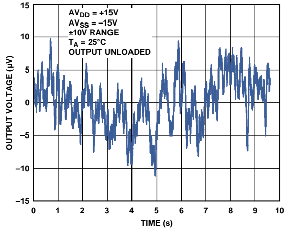
Figure 28. Peak-to-Peak Noise (0.1 Hz to 10 Hz Bandwidth)
