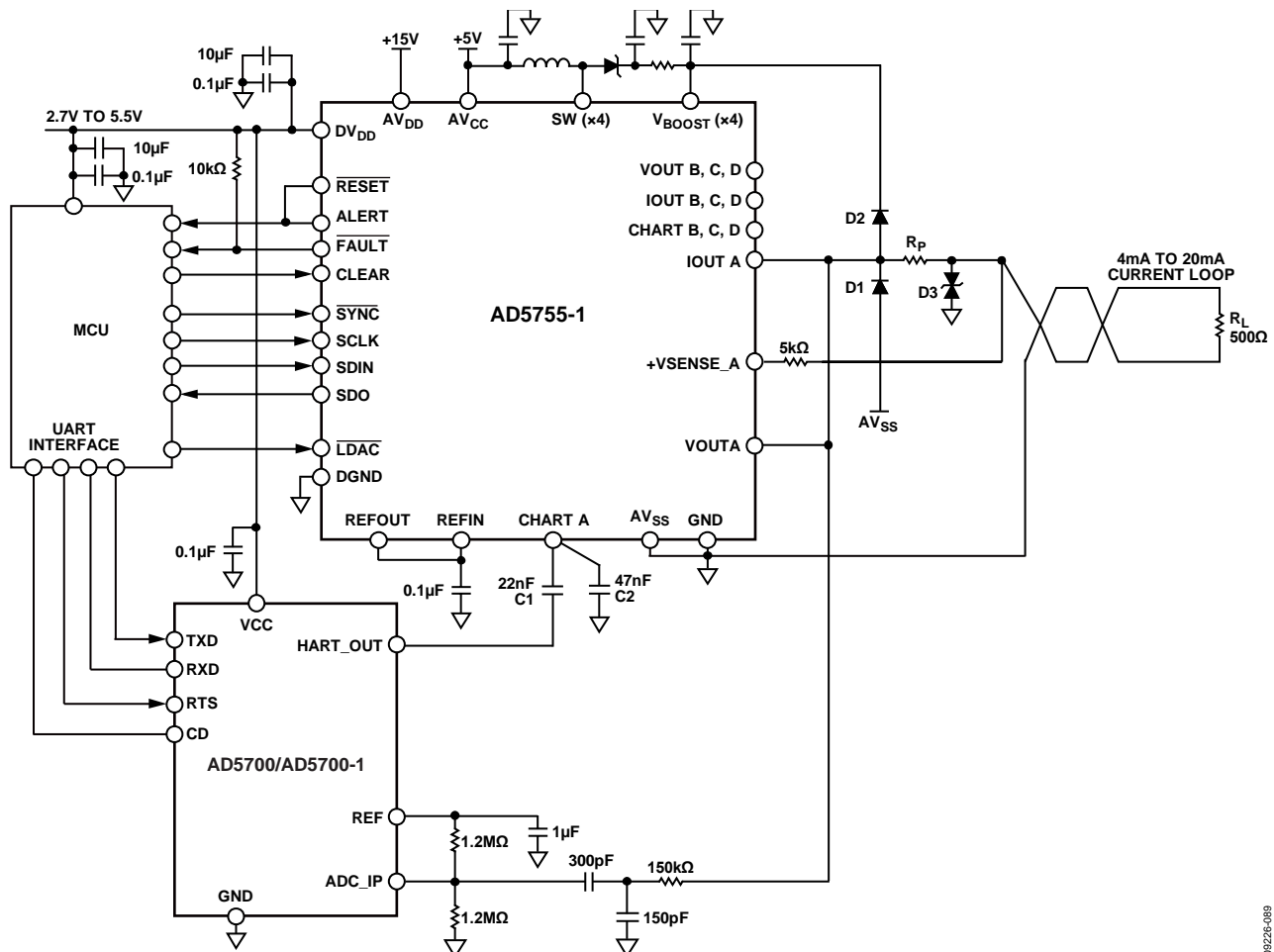
Figure 90. AD5755-1 in HART Configuration
