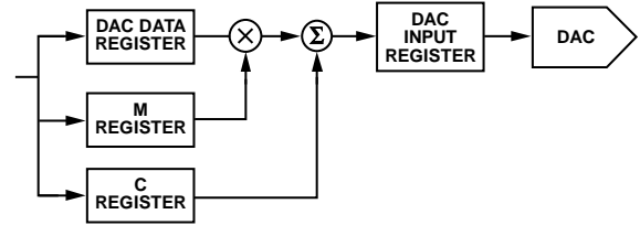
Figure 78. Digital Offset and Gain Control
