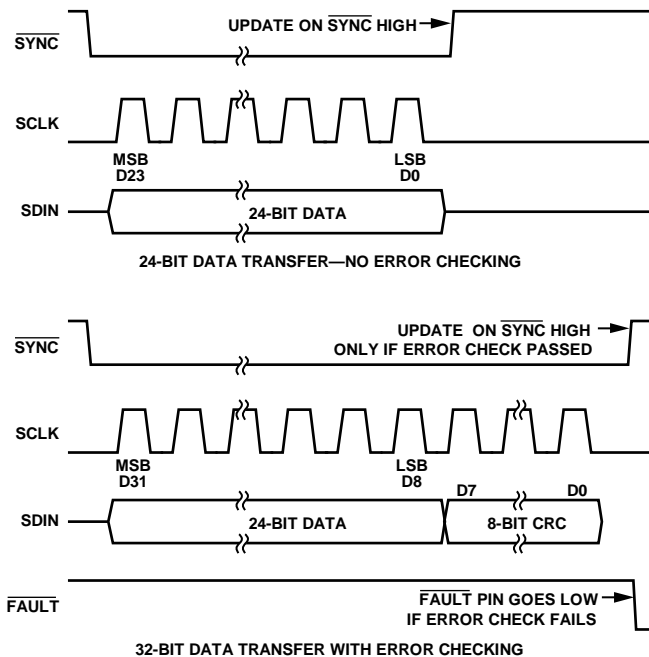
Figure 79. PEC Timing
